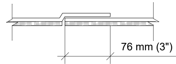
CUT A-A Side laps
