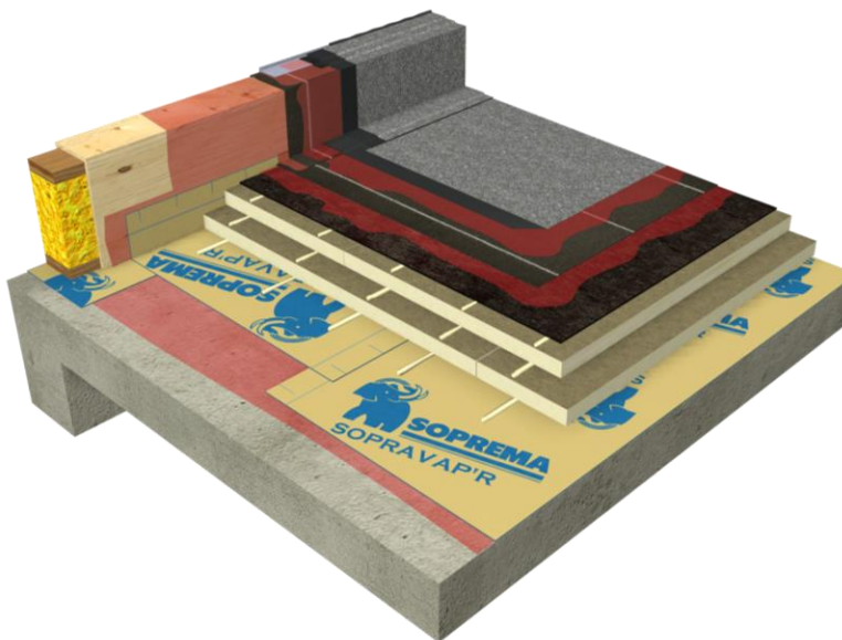
Figure 2: Self-adhered SBS modified bitumen roof membrane system example
