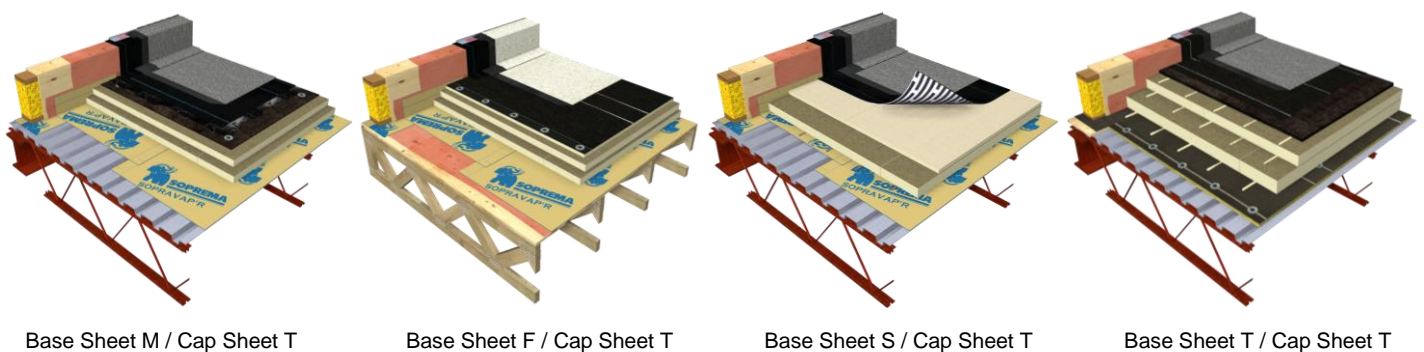
Figure 2: SBS modified bitumen roof membrane system examples with torched cap sheet
